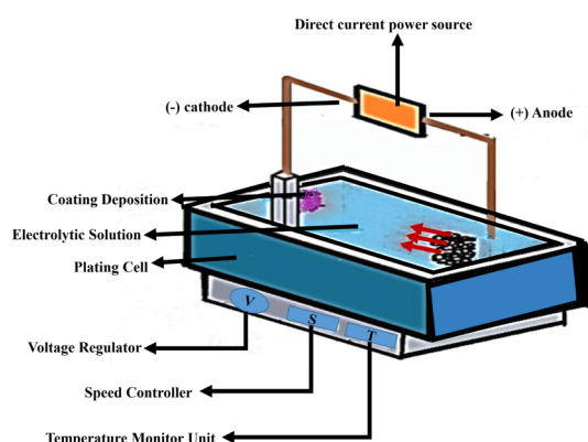
Fig. 1. Schematic of electrochemical deposition of nanocomposite on the metal surface.
