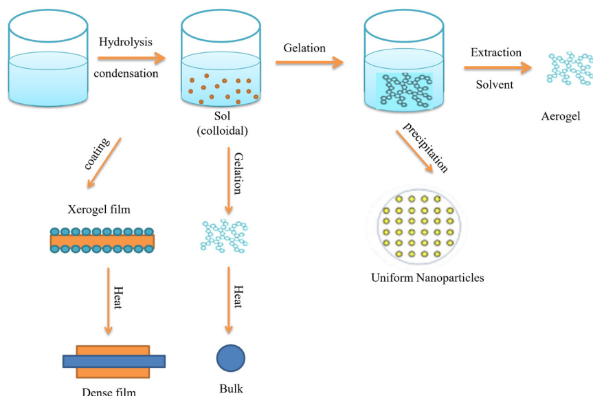
Fig. 3. Schematic illustration of sol-gel technique.
