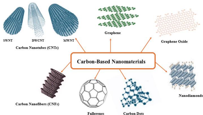
Fig. 2. Carbon-based nanomaterials.
