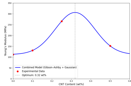
Fig. 2. Predicted Young's modulus of MWCNT-reinforced 45S5 bioglass scaffolds as a function of CNT content (wt.%), based on the combined Gibson–Ashby and Gaussian reinforcement model. Experimental data points (red circles) are from Touri et al.[14].
