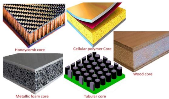
Fig. 3. Sandwich composites with various core models [16].
