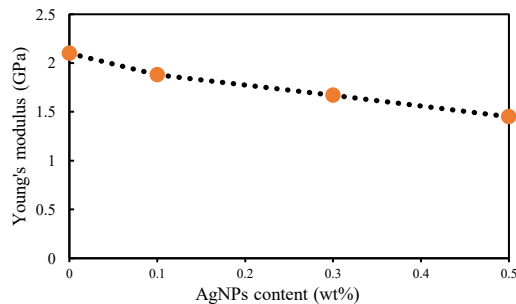
Fig. 1. The effect of AgNPs on the Young's modulus of PVC nanocomposite.
