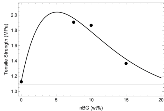
Fig. 1. Tensile strength vs. nBG content.
