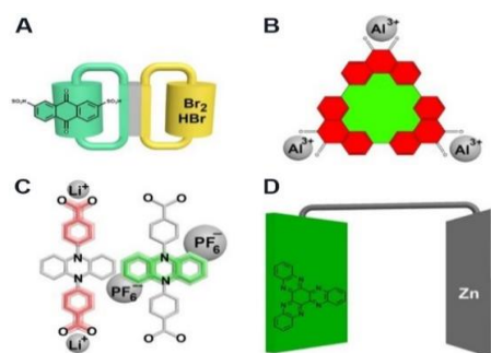
Fig. 1. Formula for the structure of certain inexpensive organic electrode materials. (A) For flow batteries, 9,10-anthraquinone-2,7-disulfonic acid. (B) A triangular macrocycle based on phenanthrenequinone that is redox active. Phenazine-5,10-diyl) dibenzoate, 4,4-. (D) The Zn-organic battery's phenazine component [28].
