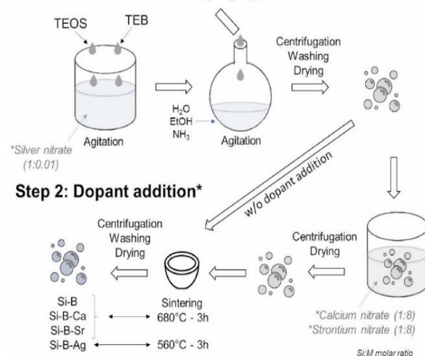
Fig. 2. Scheme of the sol-gel synthesis of Bioactive glass powders [78].
