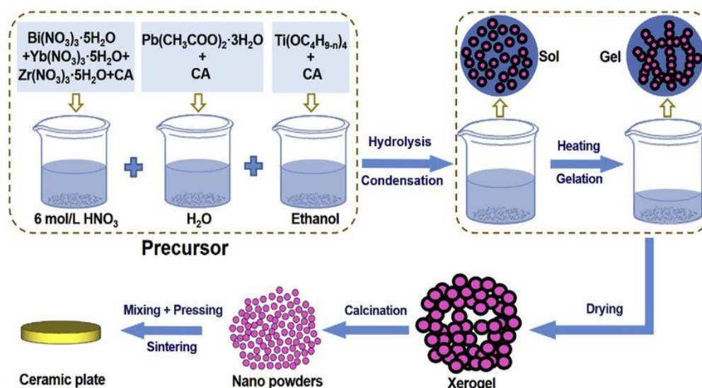
Fig. 4. Scheme of the sol-gel synthesis of ceramics [173].
